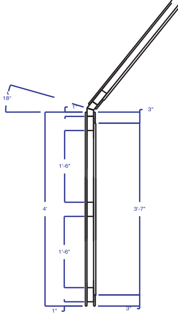
Top View Exterior side
