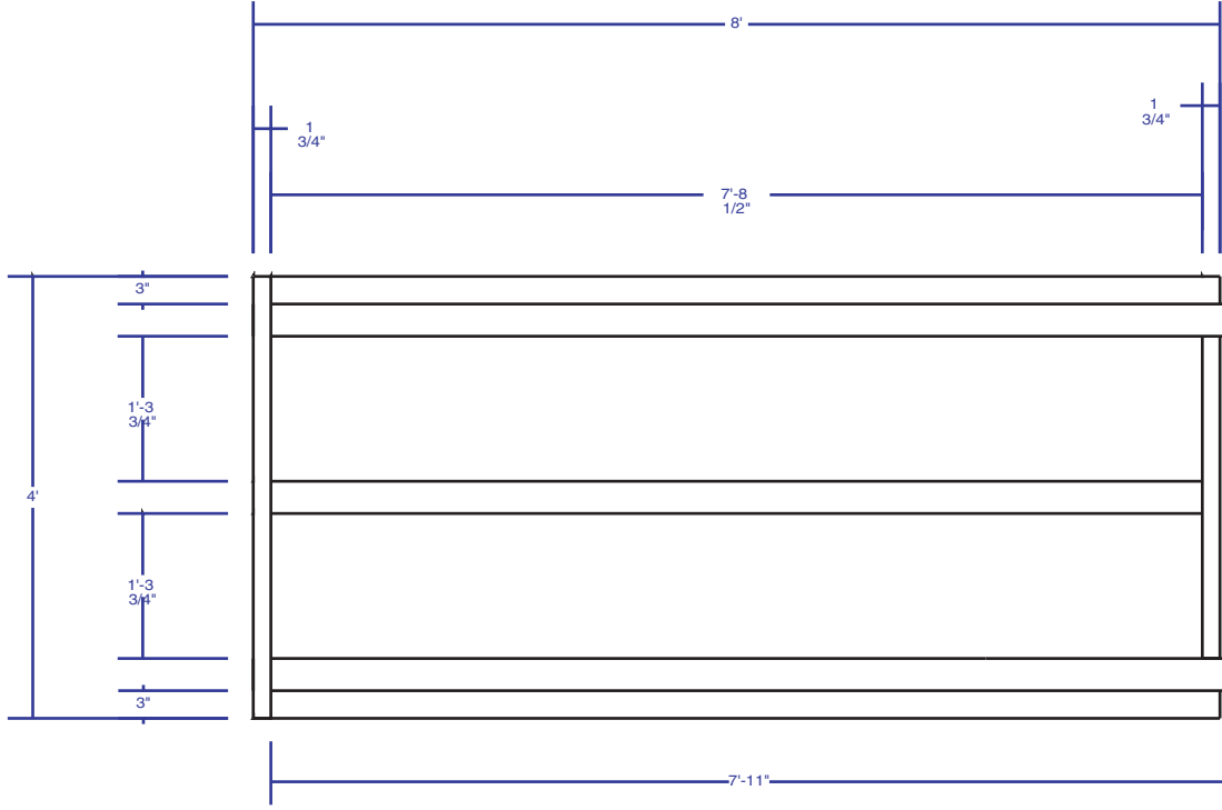
Interior section view to show 2x4 placement (with interior pinboard removed)
